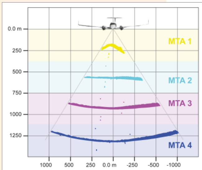
Example for a profile of scan data processed in MTA zones 1 to 4
